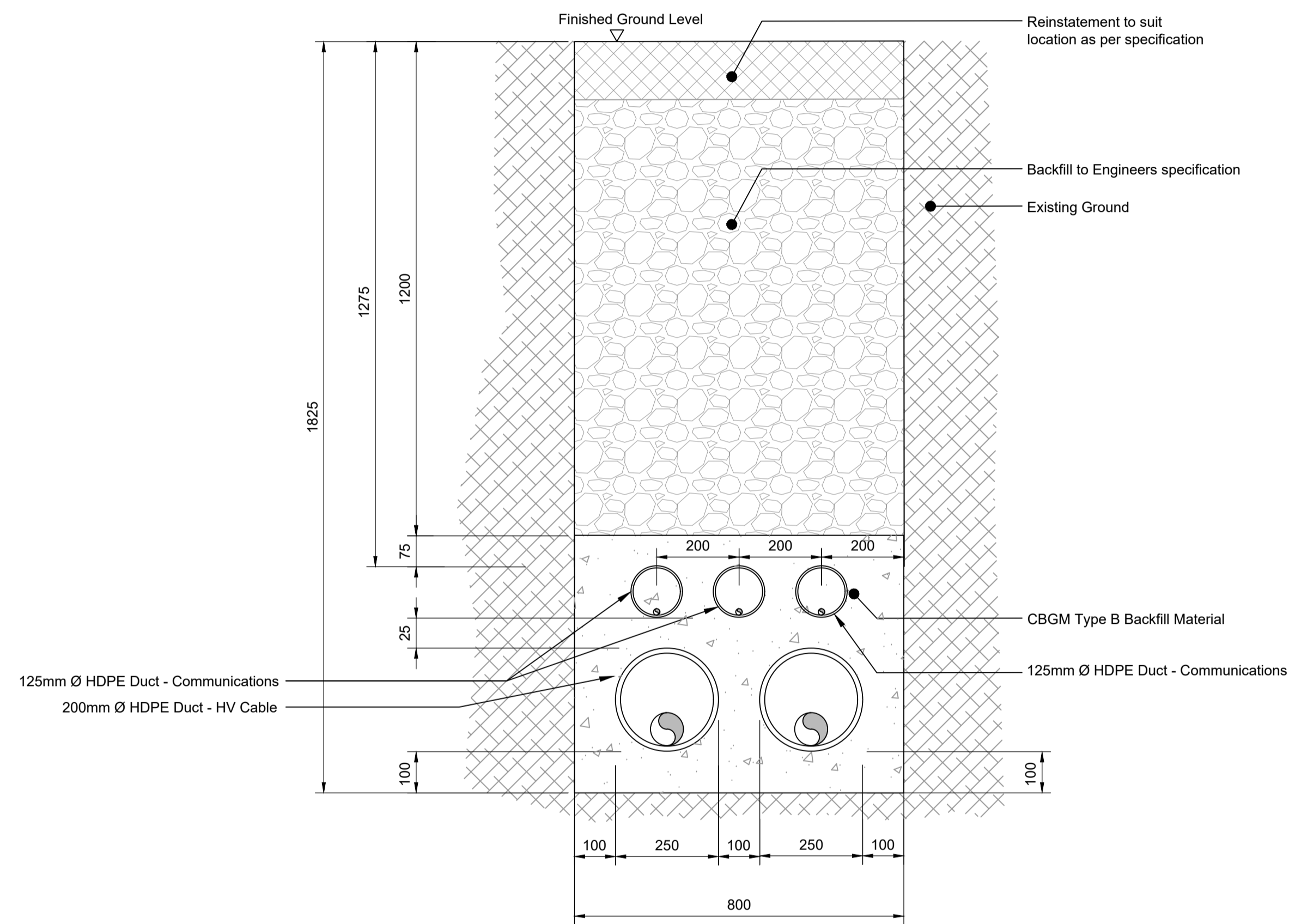
DC Cable - Typical Section 1:10
